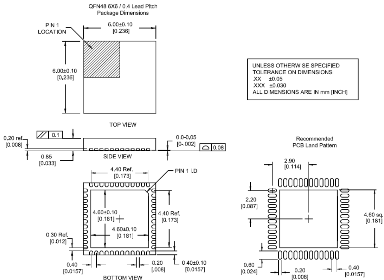
Figure 67: Package Dimensions
