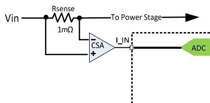
Figure 20 Input Current Sensing
