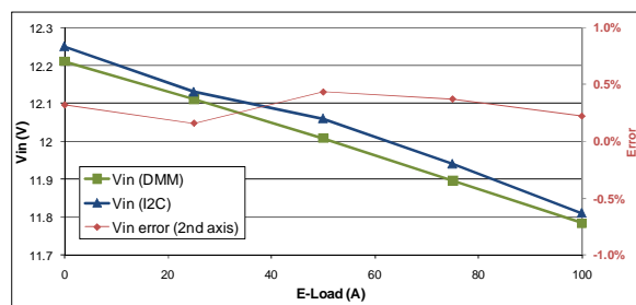
Figure 46: I2C Input Voltage Measurements
