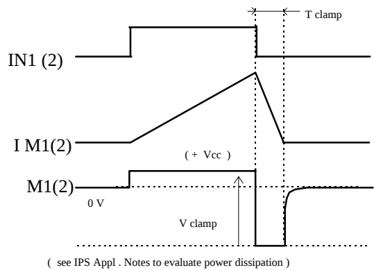
Figure 1 - Active clamp waveforms
