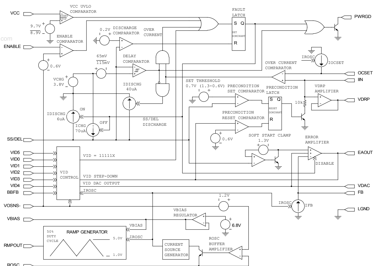
Figure 6. IR3081A Block Diagram
