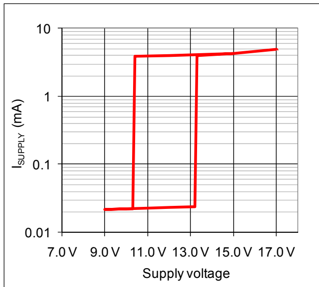
Figure 1: Supply Current vs. Supply Voltage
