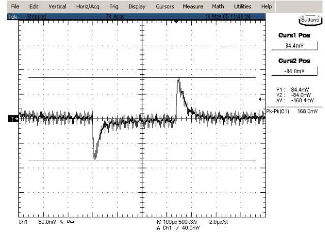
Figure 14: Typical transient response to step load change at 0.5A/\mu s from 50% to 100% of I_o , max at 36Vin, 6.5V out (measurement with a 1 \mu F ceramic)
