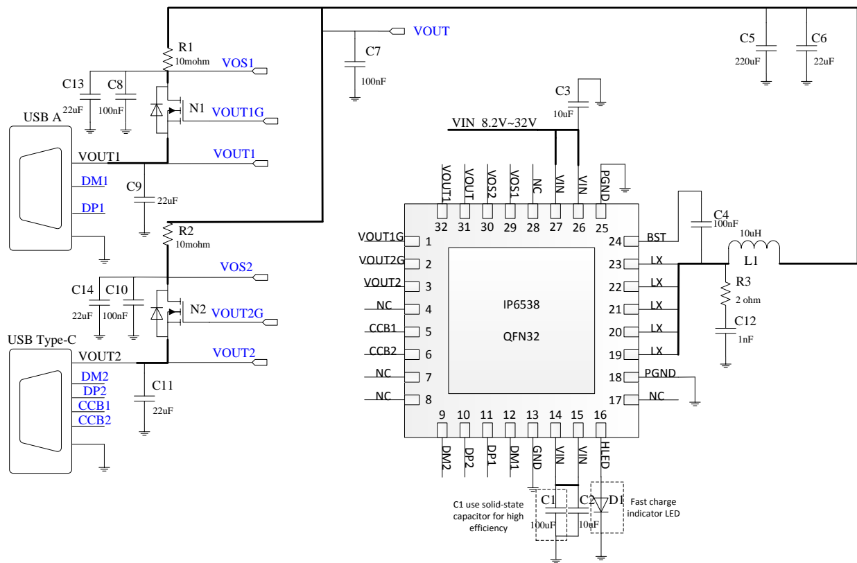
Figure 7. IP6538_AC USB A plus USB Type-C output ports fast charge application schematic diagram
