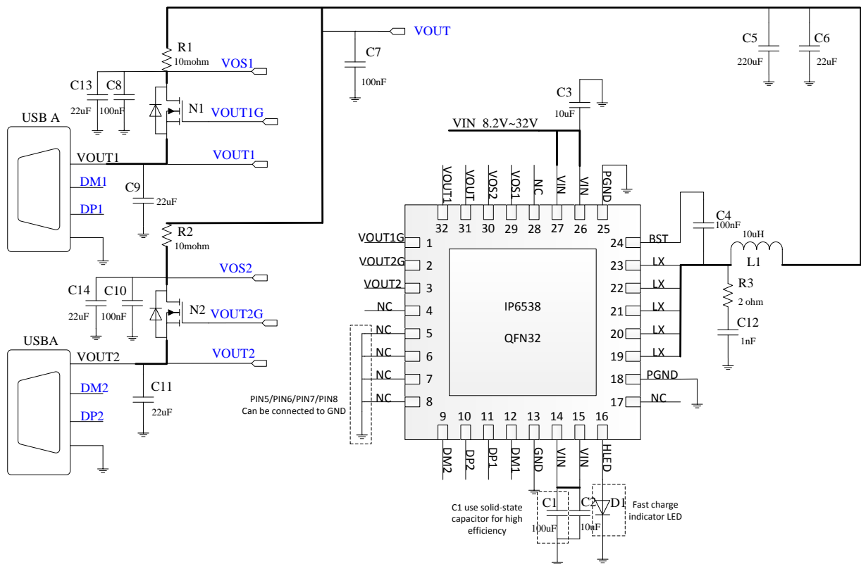
Figure 8. IP6538_AA dual USB A output ports fast charge application schematic diagram
