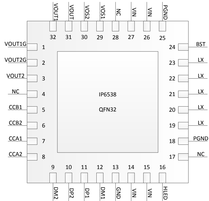
Figure 2. Pin Functions
