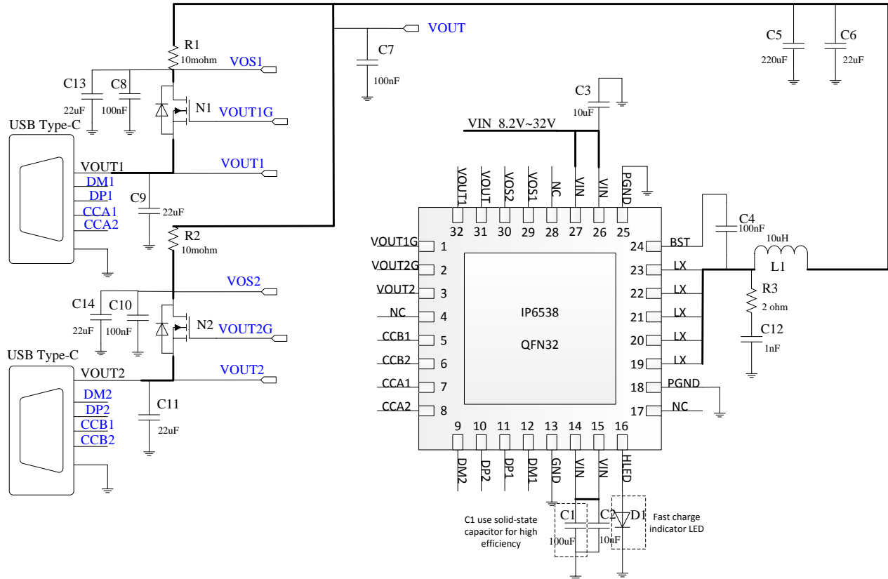
Figure 6. IP6538_CC dual USB Type-C output ports fast charge application schematic diagram
