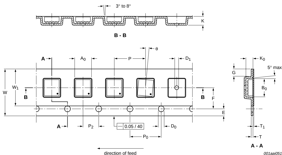
Fig 8. Tape and reel information
