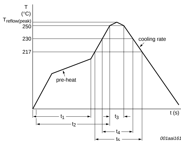
Fig 9. Pb-free solder reflow profile
