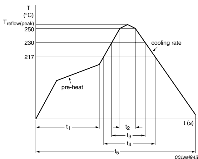
Fig 8. Pb-free solder reflow profile
