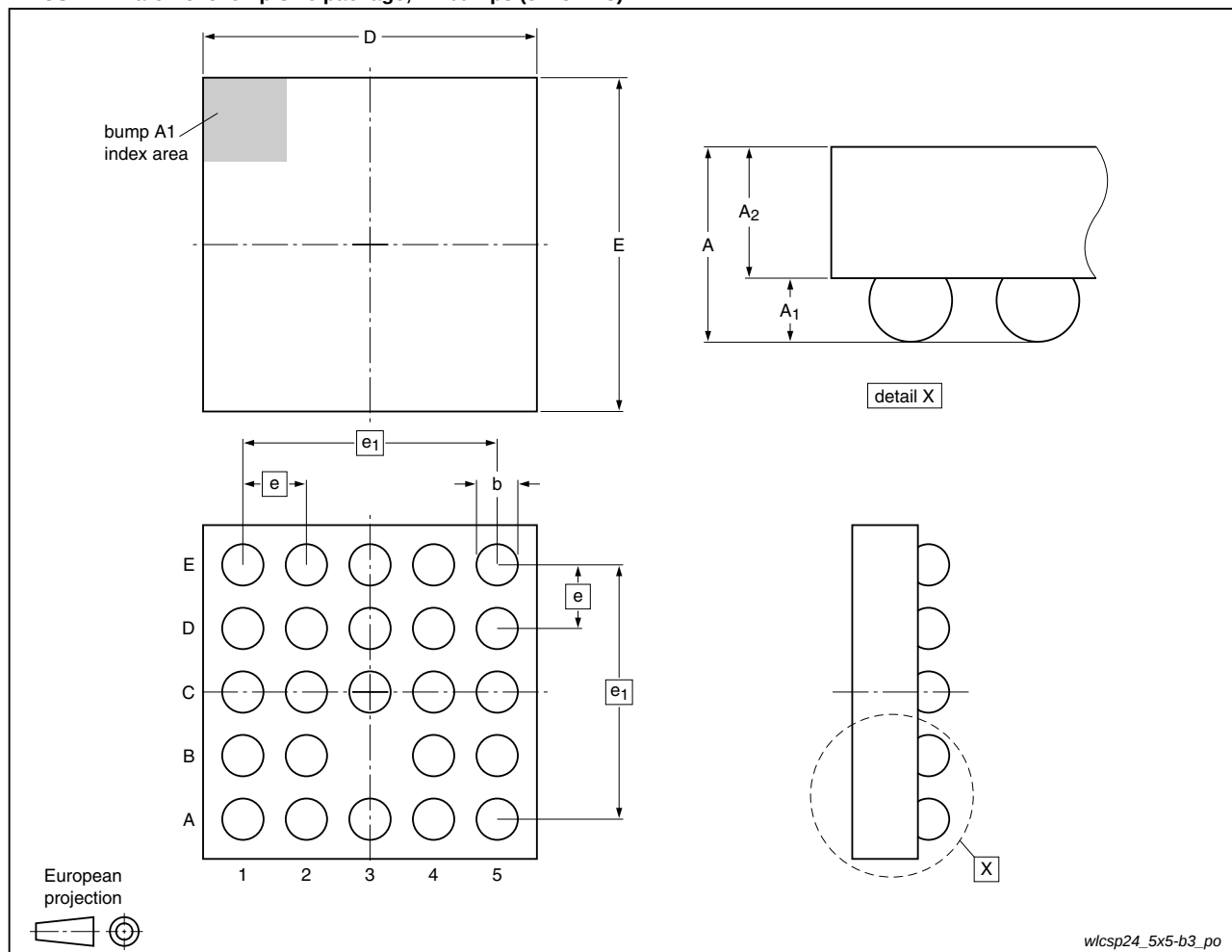
Fig 7. Package outline IP4352CX24 (WLCSP24)
