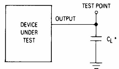
Figure 2. Test Circuit
