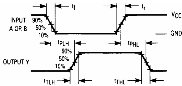
Figure 1. Switching Waveforms
