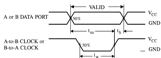
Figure 7. Switching Waveforms
