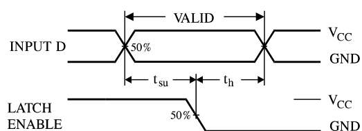
Figure 4. Switching Waveforms
