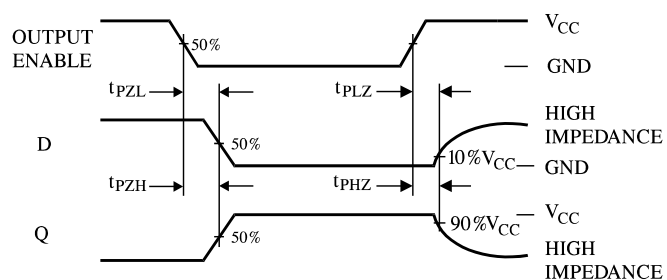
Figure 3. Switching Waveforms
