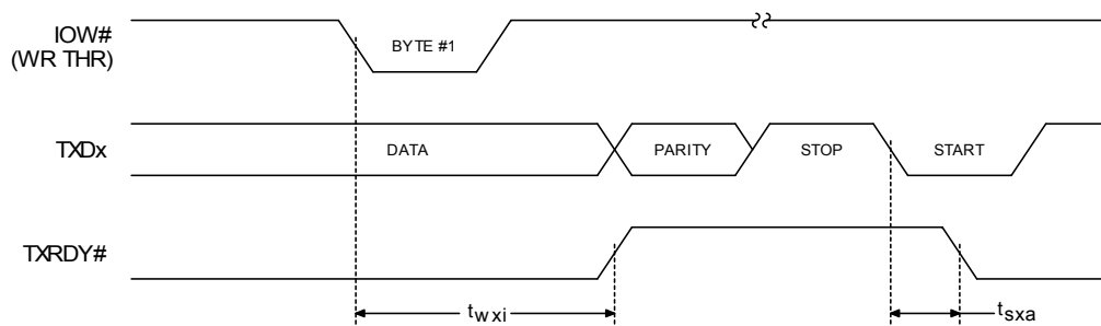
Figure 13: Transmitter Ready Mode 0 Timing
