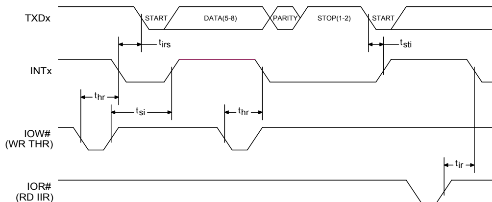
Figure 12: Transmitter Timing
