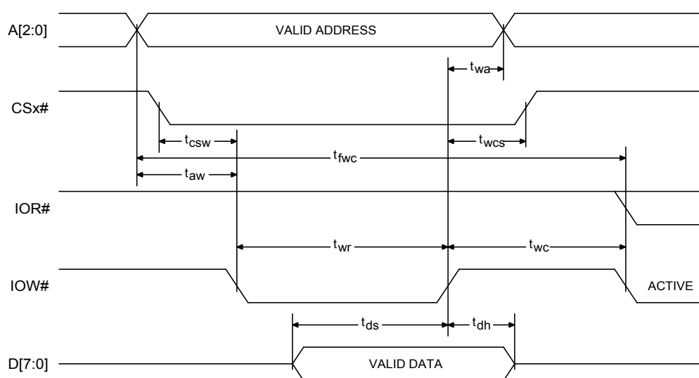
Figure 11: Write Cycle Timing
