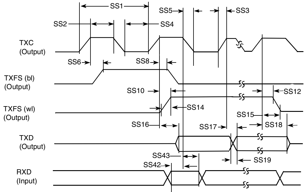
Figure 92. SSI Transmitter Internal Clock Timing Diagram
