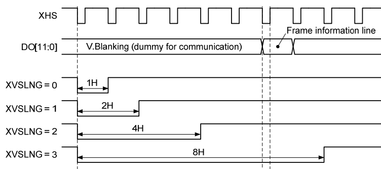
List of XVS Pulse Width Setting
