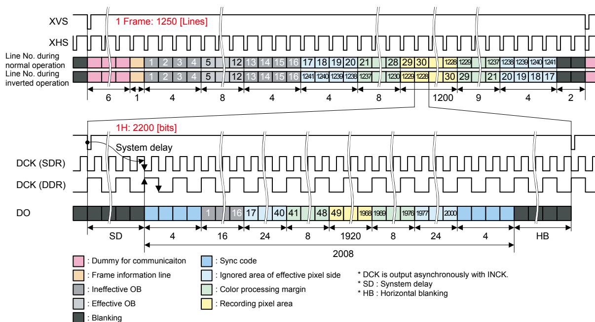
Drive Timing Chart for Parallel CMOS Output in All-pixel Scan Mode
