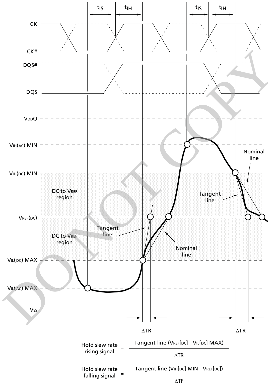
Figure 36: Tangent Line for t_{IH} (Command and Address – Clock)
