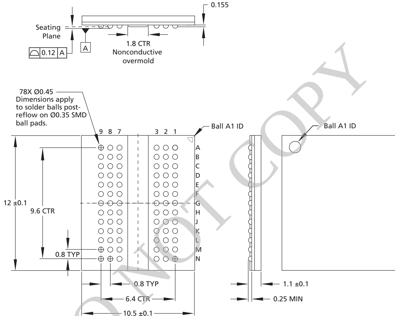
Figure 7: 78-Ball FBGA – x4, x8; “RAF”
