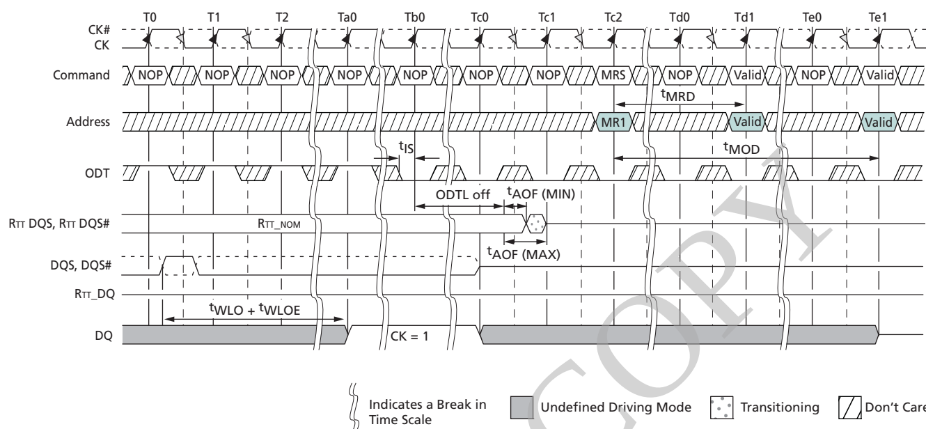
Figure 48: Exit Write Leveling
