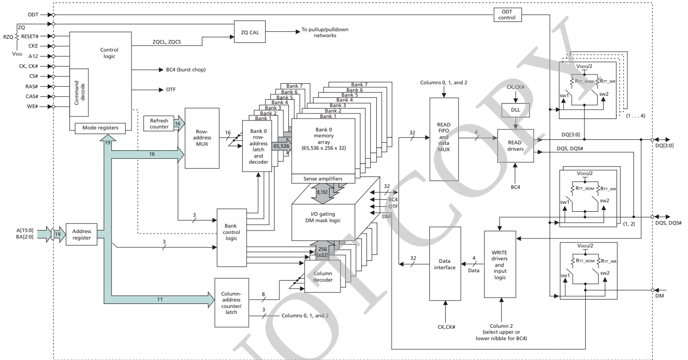
Figure 2: 1 Gig x 4 Functional Block Diagram
