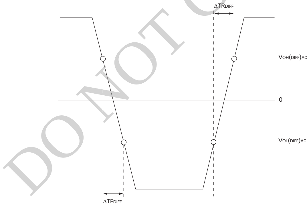
Figure 32: Nominal Differential Output Slew Rate Definition for DQS, DQS#
