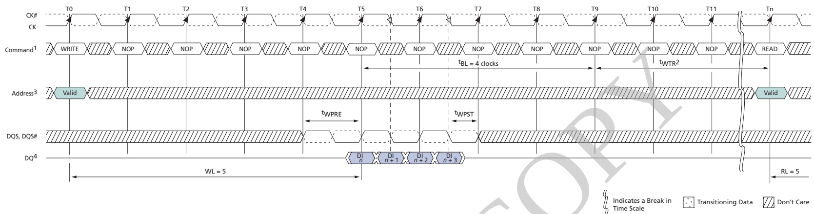
Figure 90: WRITE (BC4 OTF) to READ (BC4 OTF)
