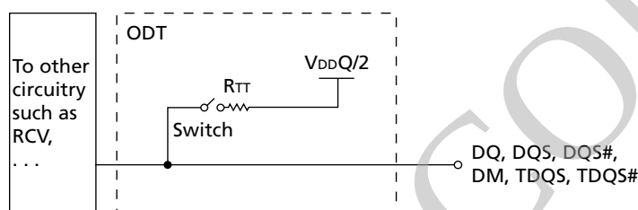
Figure 108: On-Die Termination
