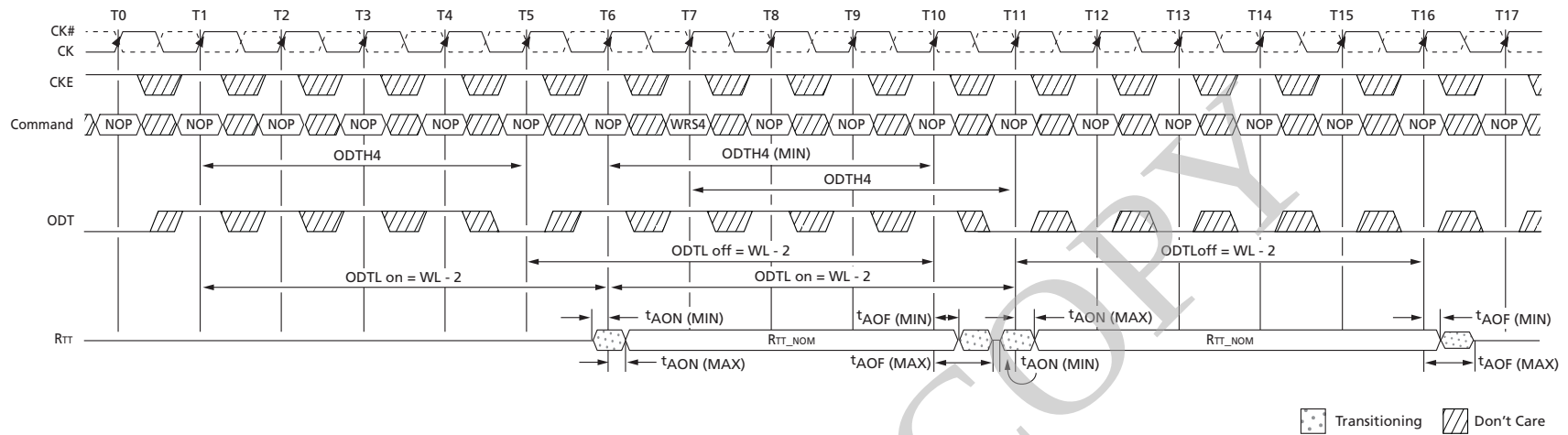
Figure 115: Synchronous ODT (BC4)
