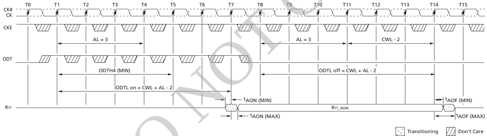
Figure 114: Synchronous ODT
