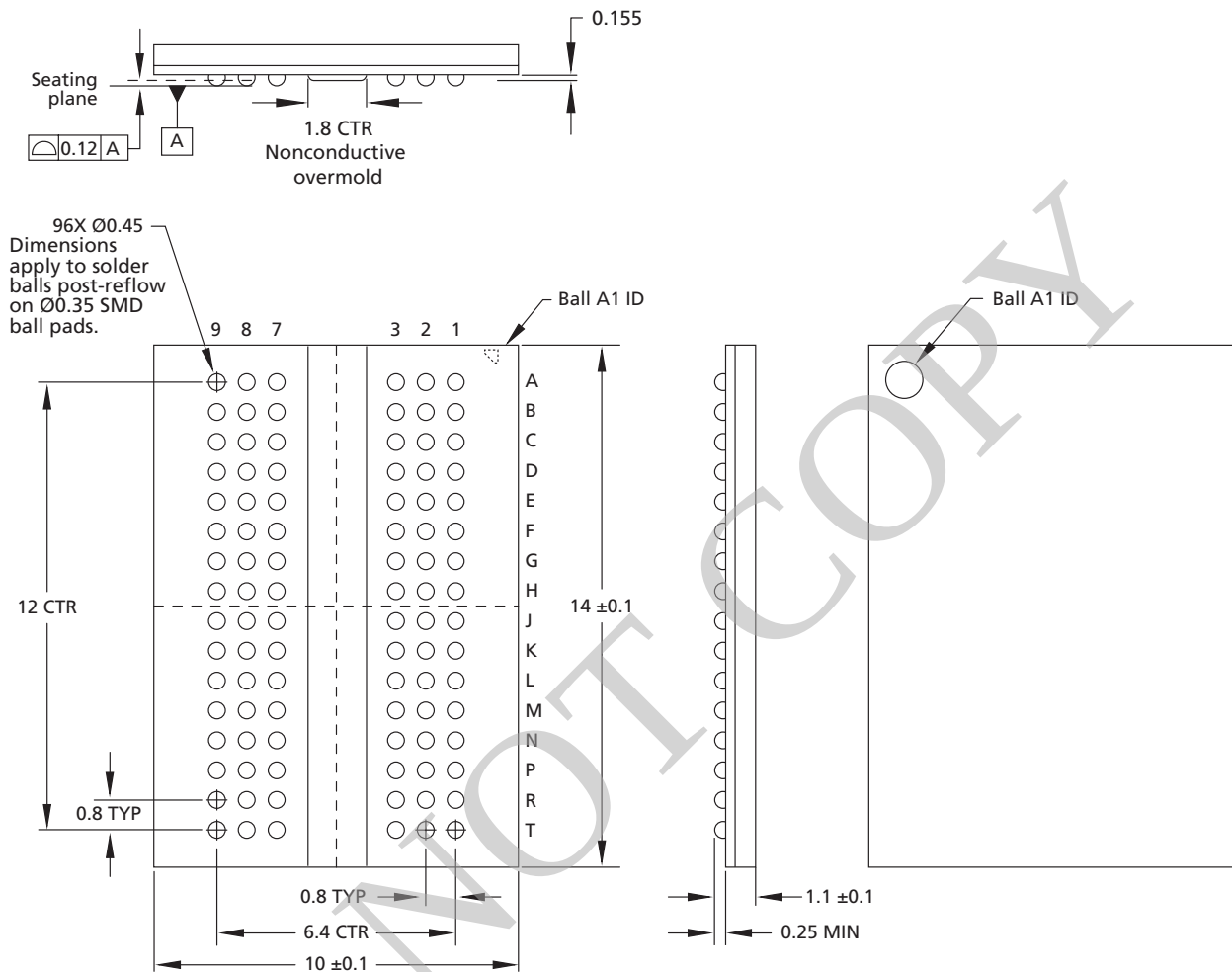
Figure 11: 96-Ball FBGA – x16; “REF”
