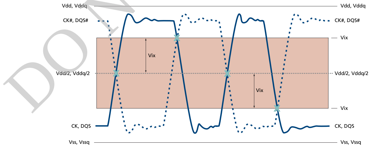
Figure 17: V_{IX} for Differential Signals
