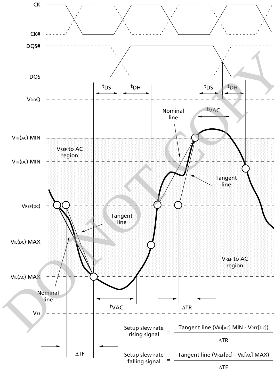
Figure 39: Tangent Line for t_{DS} (DQ – Strobe)
