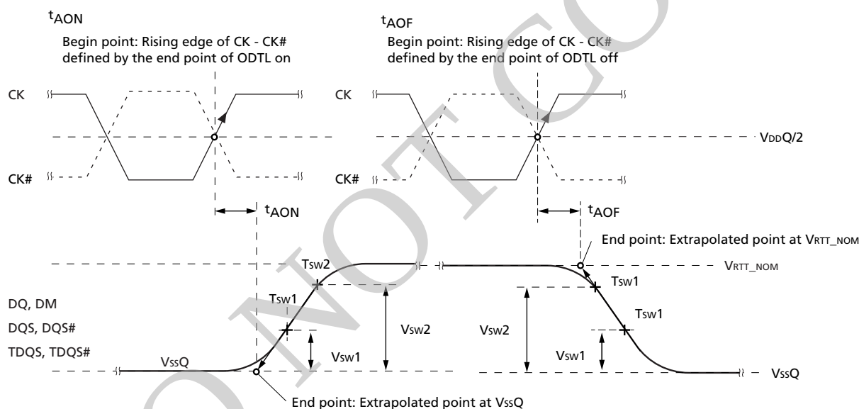
Figure 24: t_{AON} and t_{AOF} Definitions
