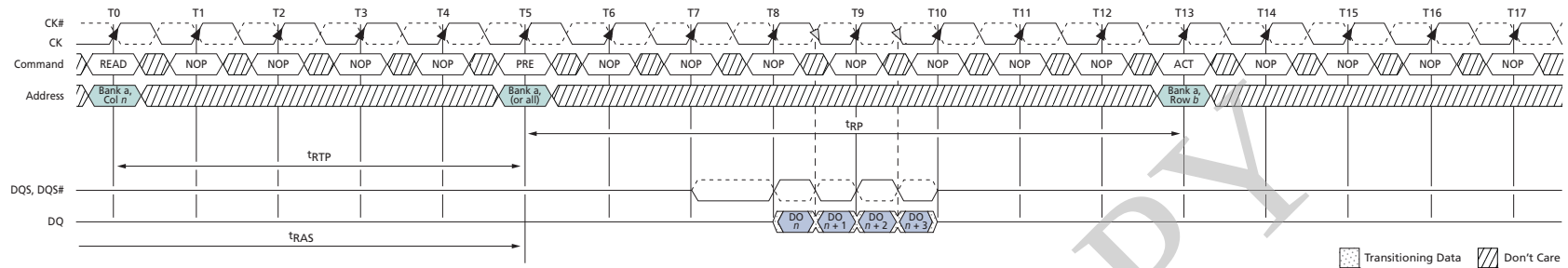
Figure 75: READ to PRECHARGE (AL = 5, CL = 6)
