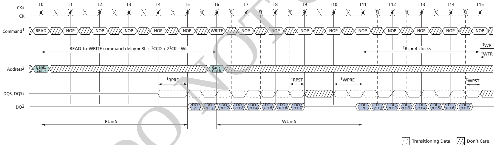
Figure 71: READ (BL8) to WRITE (BL8)
