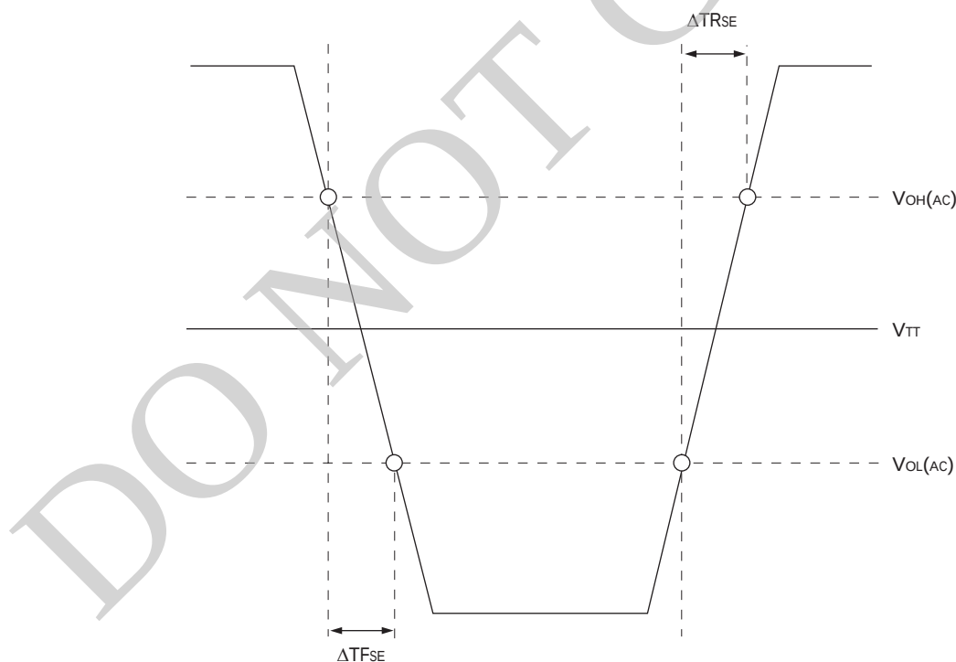
Figure 31: Nominal Slew Rate Definition for Single-Ended Output Signals
