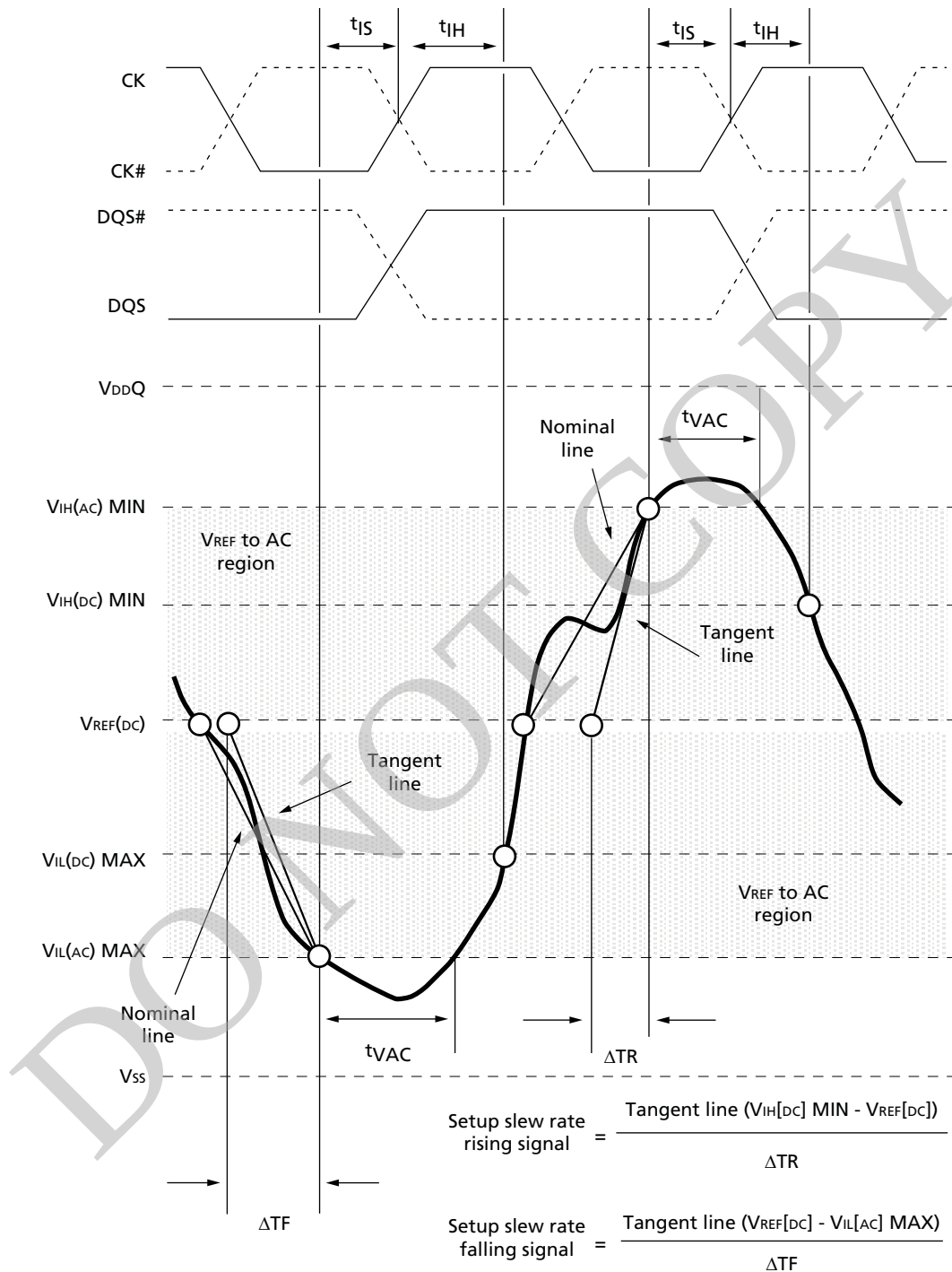
Figure 35: Tangent Line for t_{IS} (Command and Address – Clock)
