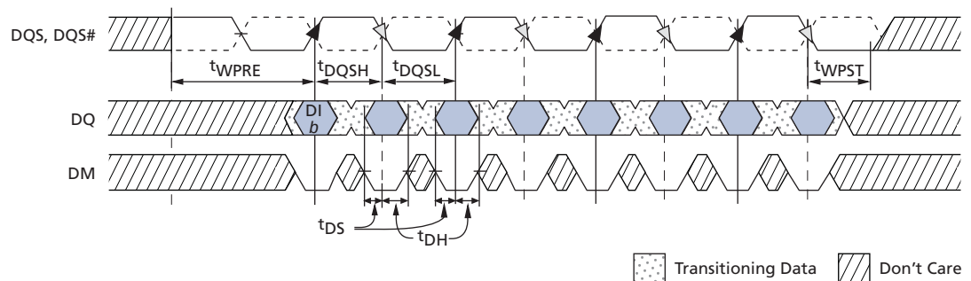
Figure 94: Data Input Timing
