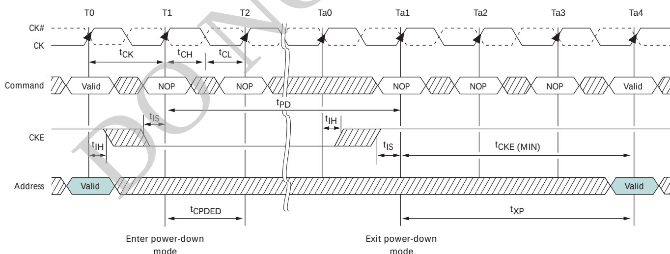
Figure 96: Active Power-Down Entry and Exit
