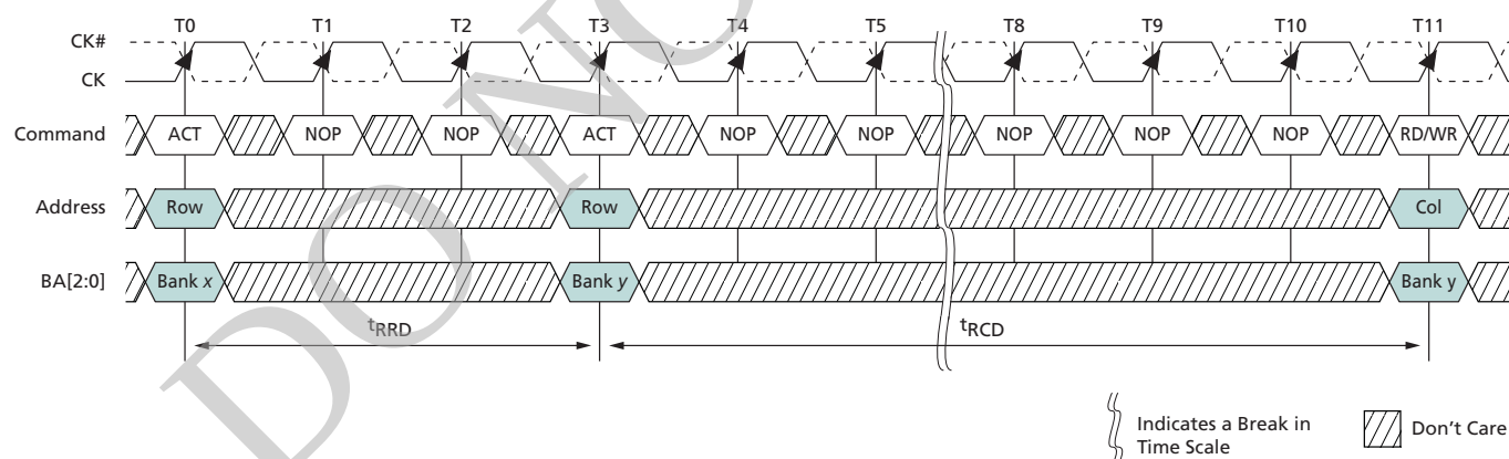
Figure 65: Example: Meeting t_{\text{RRD}} (\text{MIN}) and t_{\text{RCD}} (\text{MIN})
