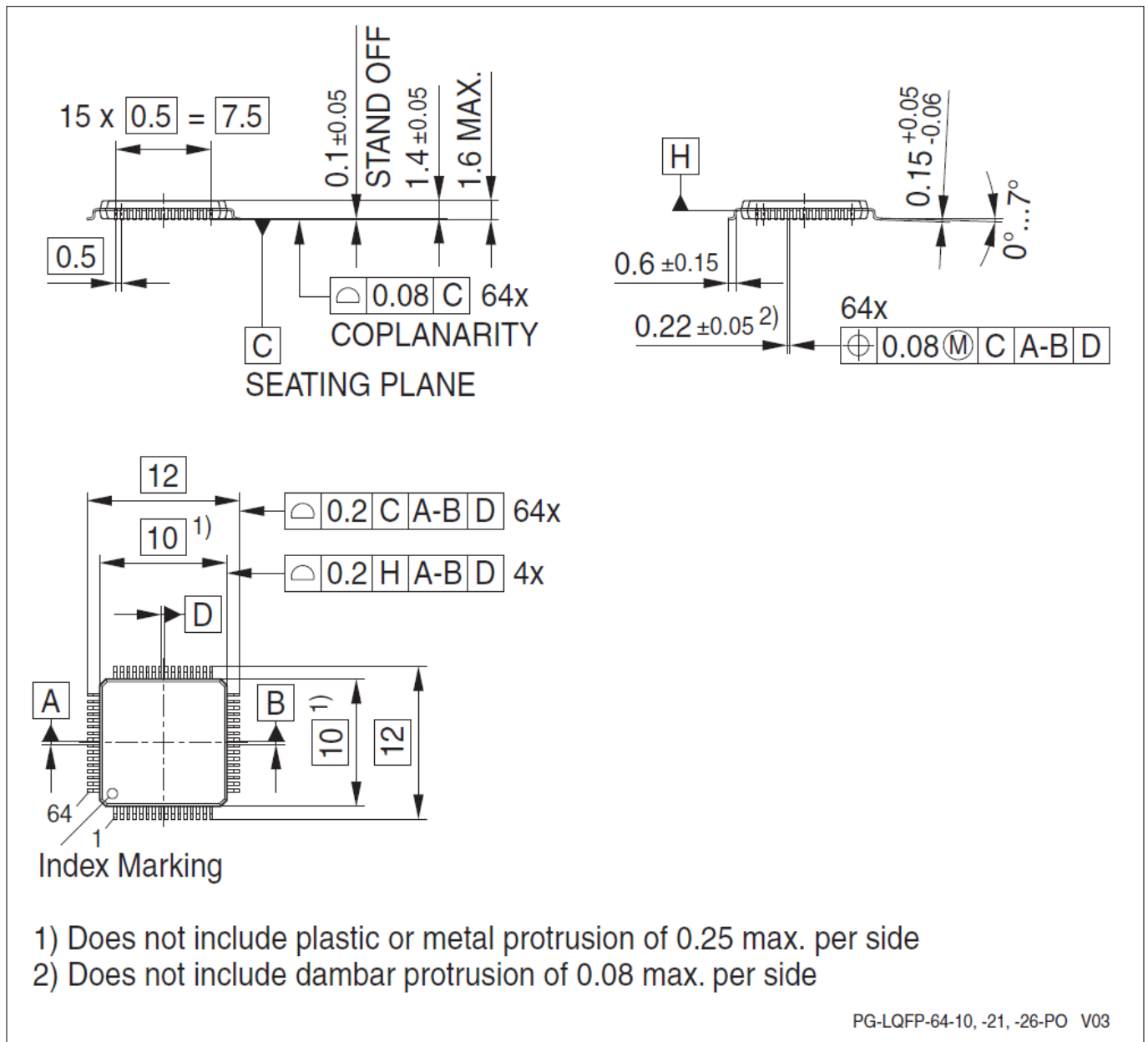
Figure 26 PG-LQFP-64-26
