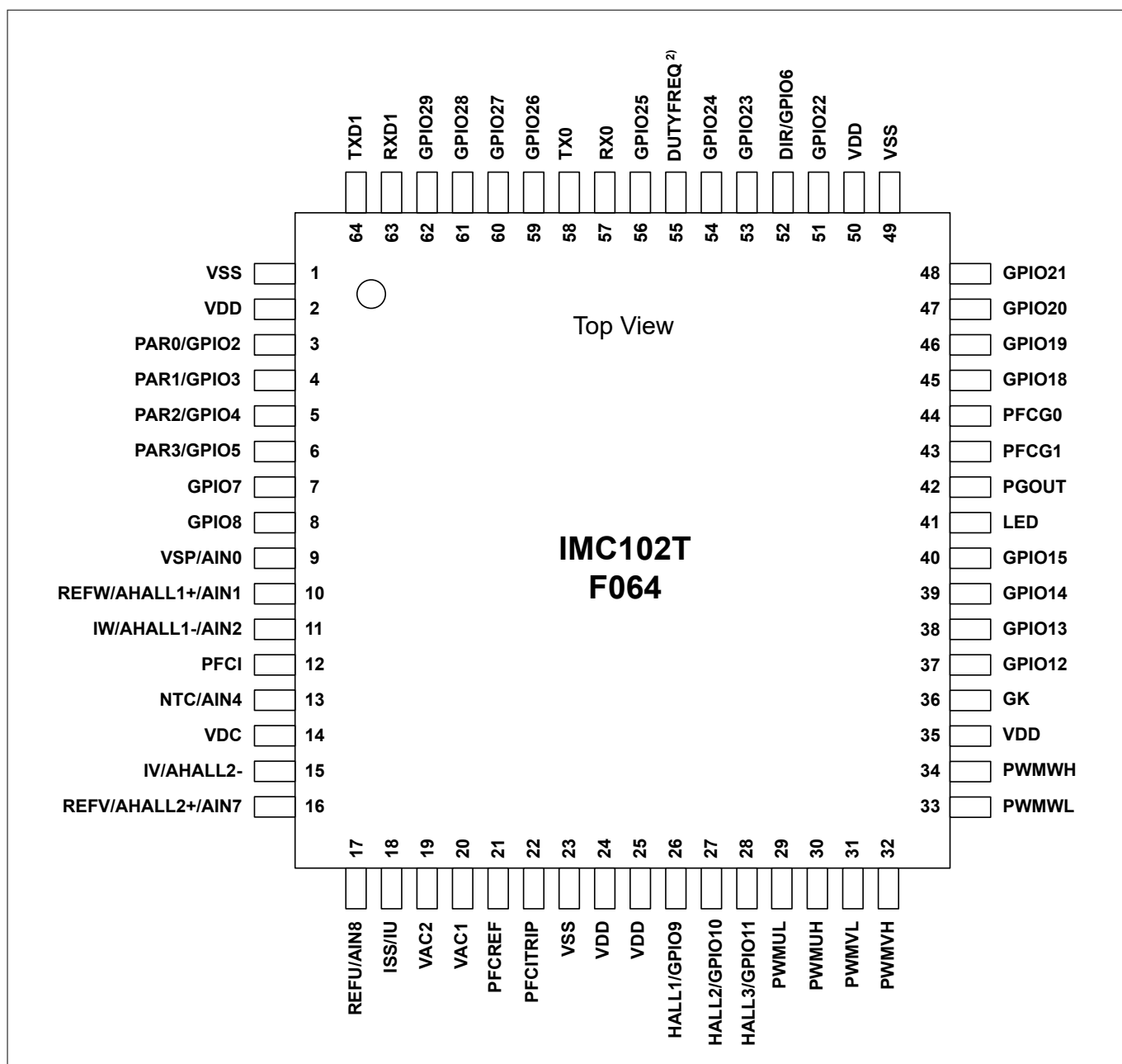
Figure 8 IMC102T-F064
