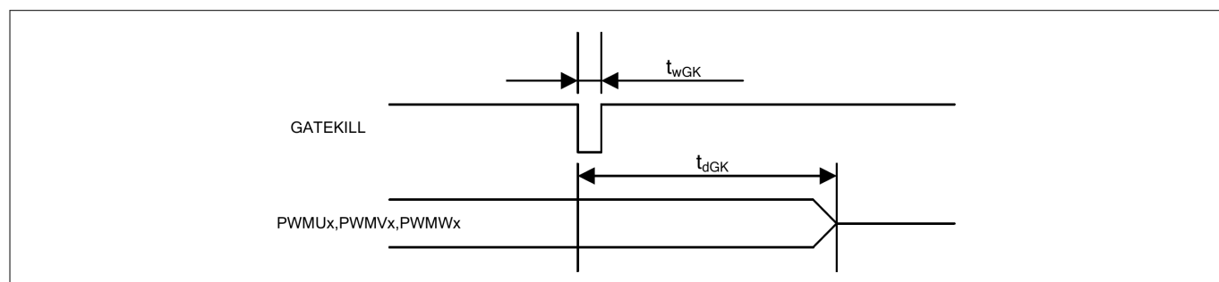
Figure 18 Fault timing
