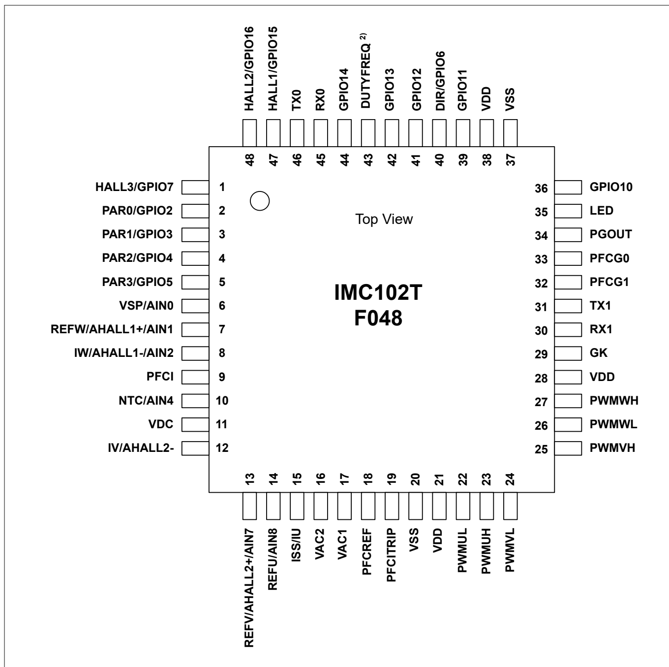
Figure 7 IMC102T-F048
