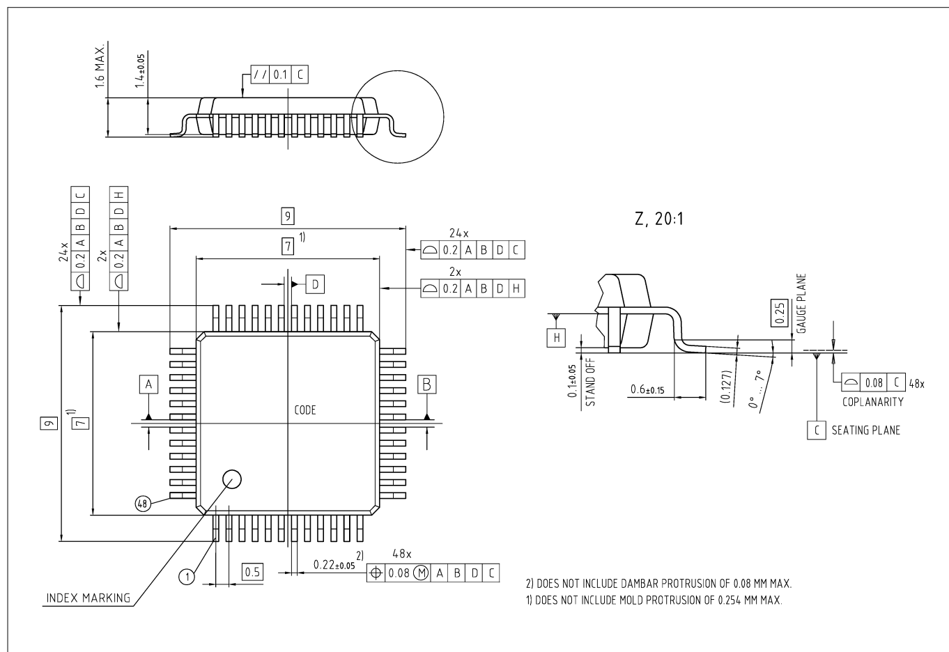
Figure 25 PG-LQFP-48-10
