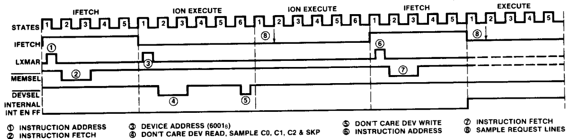
Figure 13: Interrupt Enable FF ON (ION)
