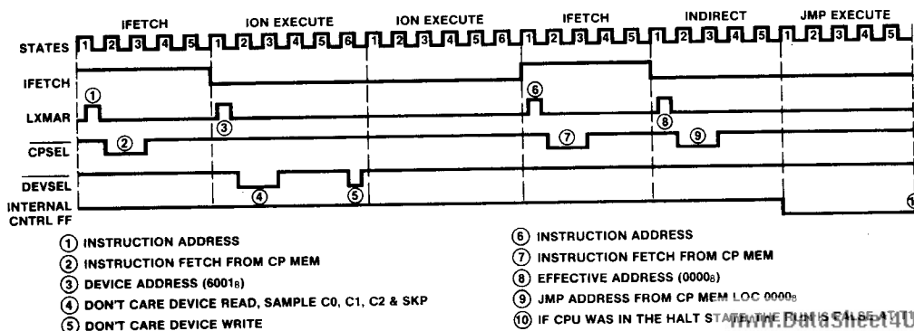
Figure 16: "ION; JMP I 0000 8 " In Control Panel Routine
