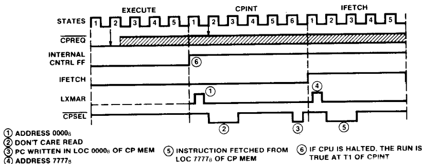
Figure 14: Control Panel Interrupt Grant Timing
