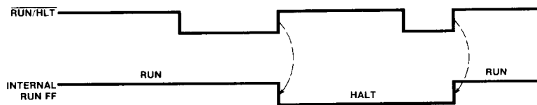
Figure 20: Run/Halt Timing
