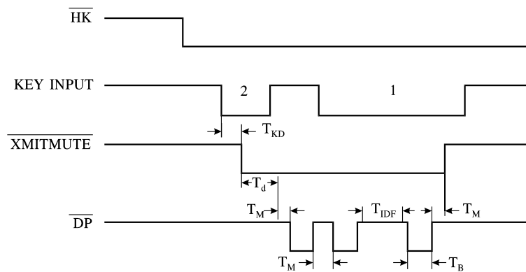
Figure 1. Pulse Mode
