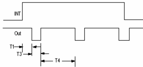
Figure 2. Switching Waveform INT Timing
