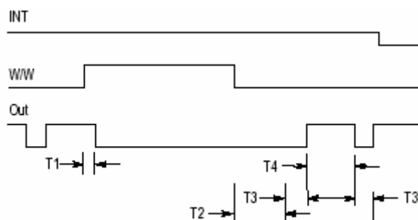
Figure 4. Switching Waveform W/W and INT Active
