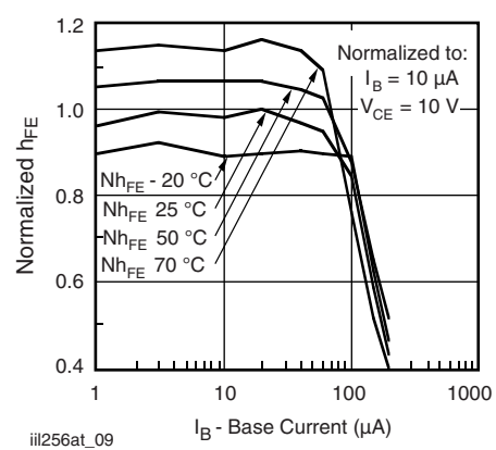
Fig. 9 - Normalized h_{FE} vs. Base Current and Temp.
