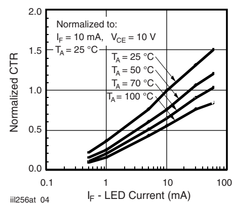
Fig. 4 - Normalized CTR vs. I_F and T_{amb}
