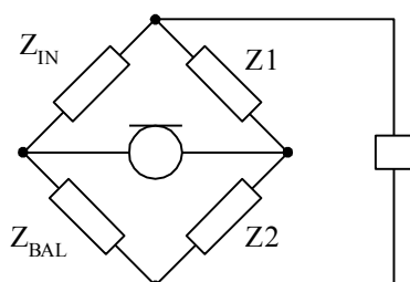
Figure 8 – Side Tone Balance
