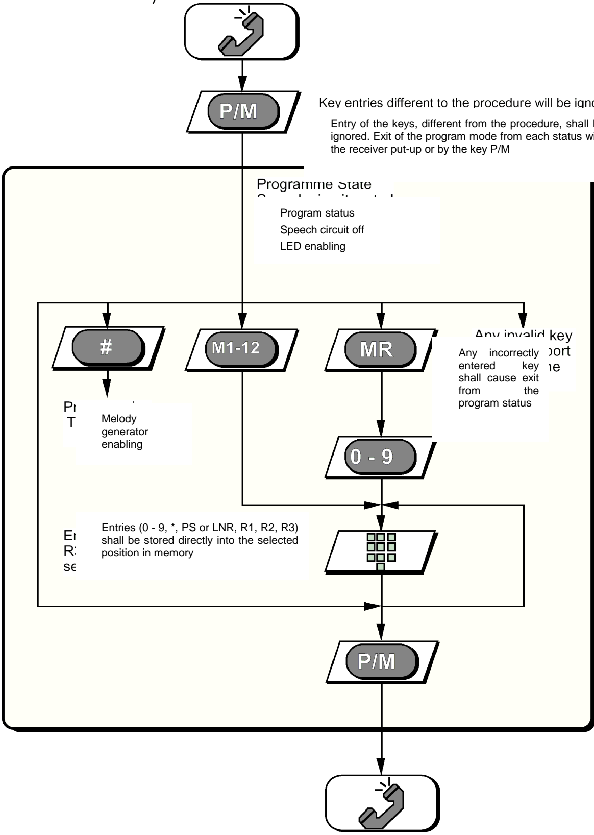
Figure 13 – Storing numbers
