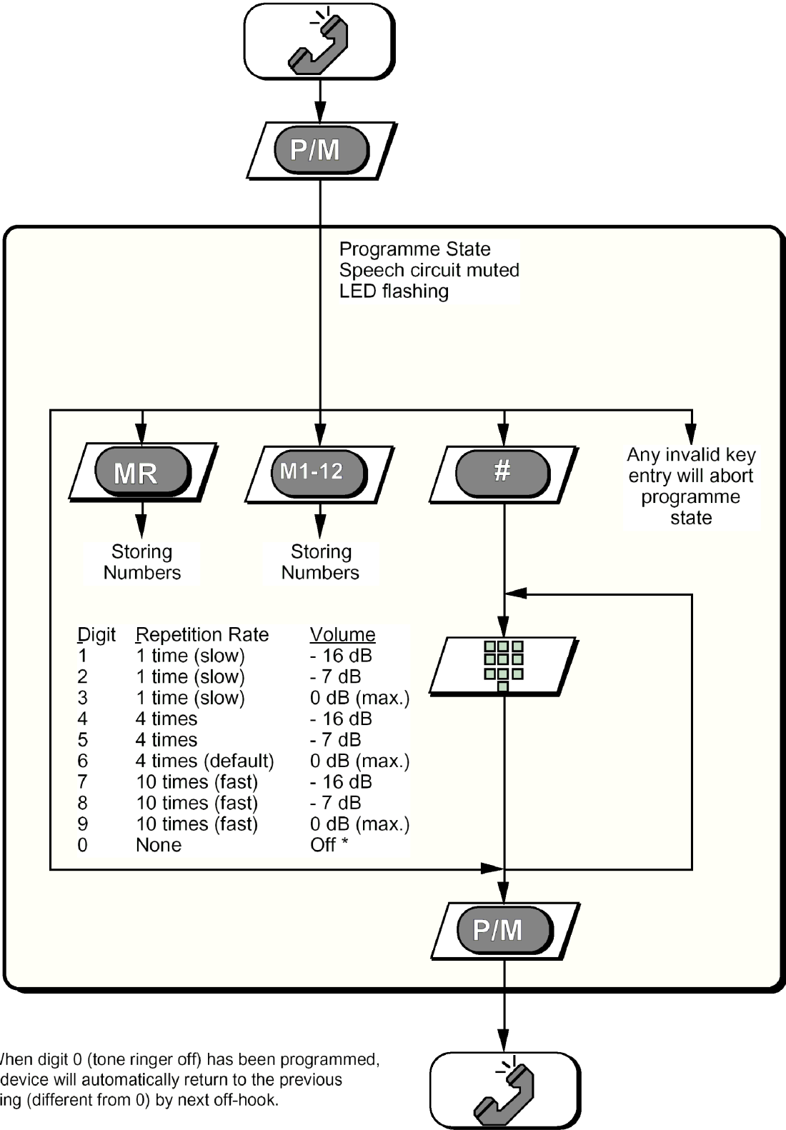
Figure 11 – Ring tone programming
