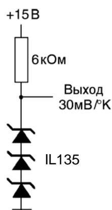
Figure 17 – Sequential sensor connection for increase of temperature bias voltage–
