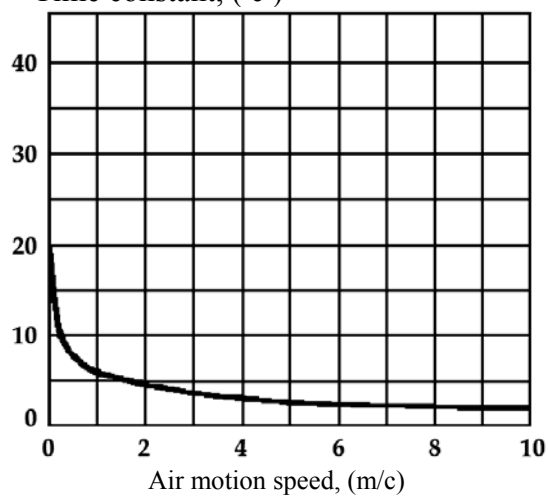
Figure 10 – Time constant versus air motion speed
