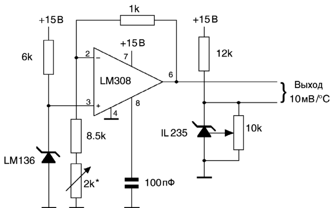
Figure 20 – Thermal sensor with 100° scale
