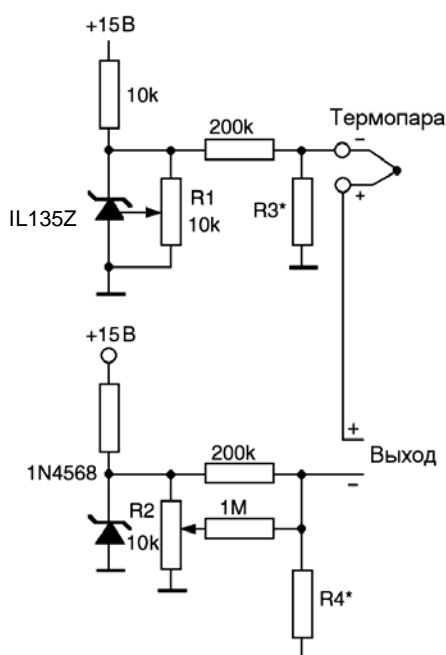
Figure 23 – Circuit of cold junction compensation with unipolar supply
