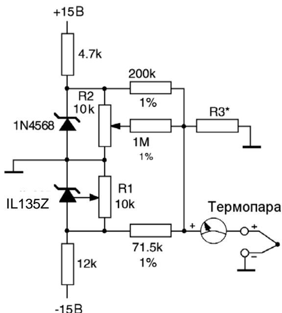
Figure 22 – Circuit of cold junction compensation (compensation for ground thermocouple)
