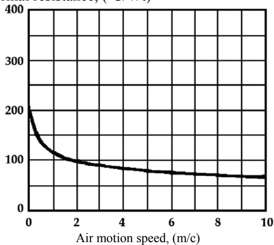
Figure 9 – Thermal resistance versus air motion speed
