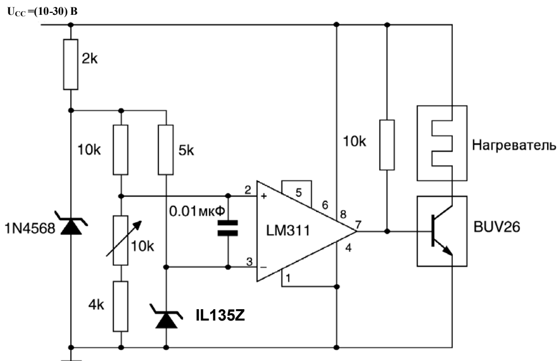
Figure 19 – Temperature regulator
