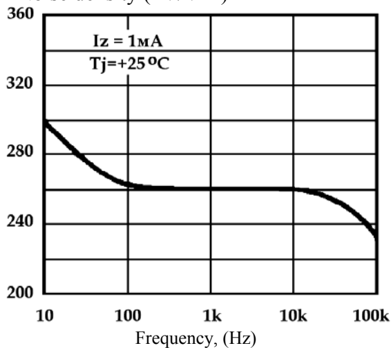
Figure 8 – Noise voltage
