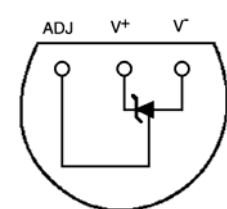
Figure 1 - Package pin definitions
