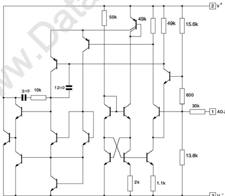
Figure 2 - circuitry IL135Z.
