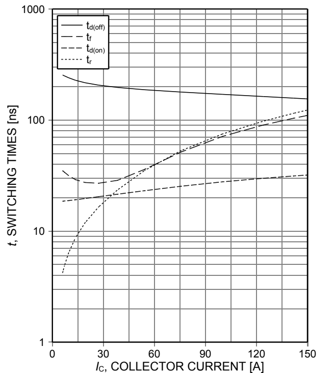
Figure 8. Typical switching times as a function of collector current (inductive load, T_j=150^\circ\text{C} , V_{CE}=400\text{V} , V_{GE}=15/0\text{V} , r_G=12\Omega , Dynamic test circuit in Figure E)
