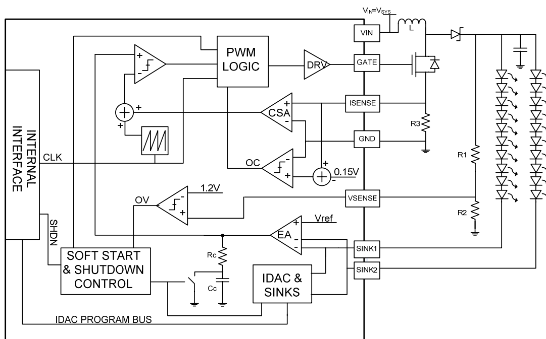
Figure 28 – White LED Boost and Sink Driver Block Diagram
