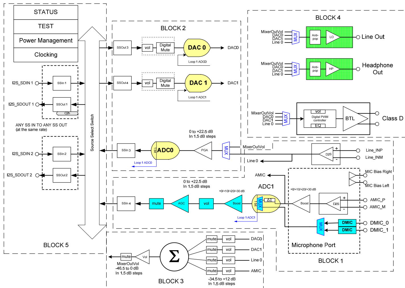
Figure 4. Audio Block Diagram
