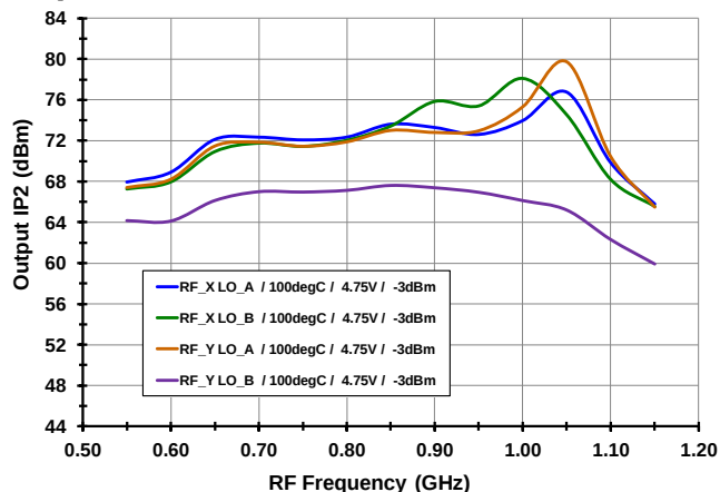
Output IP2 [High Side Injection]
