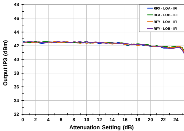
IP3 O [0.8 GHz RF, HiSide Inj.]
