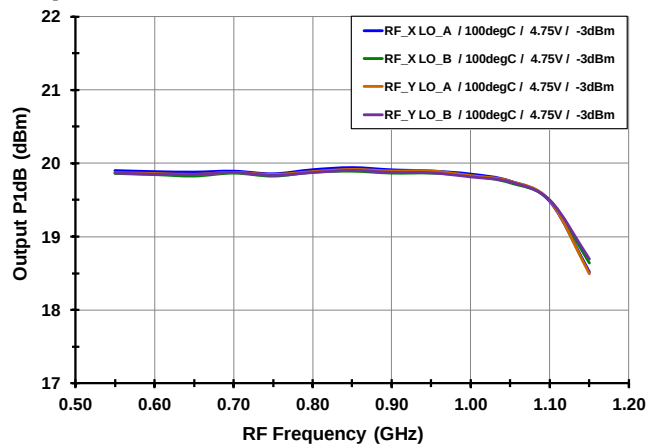
Output P1dB [High Side Injection]
