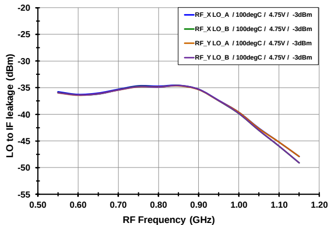
LO to IF [High Side Injection]
