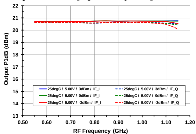
P1dB 0 vs. LO level [High Side Injection]
