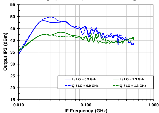
IP3 0 Flatness [High Side Injection, RF_Y LO_B]
