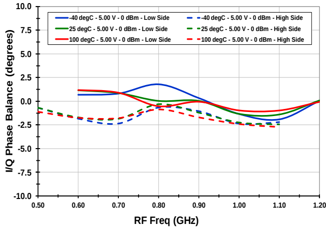
I/Q Phase Error vs. T CASE
