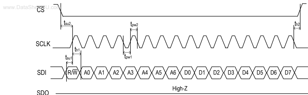
Figure 25. Serial Write Timing Diagram
