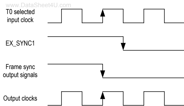
Figure 11. 0.5 UI Late Frame Sync Input Signal Timing
