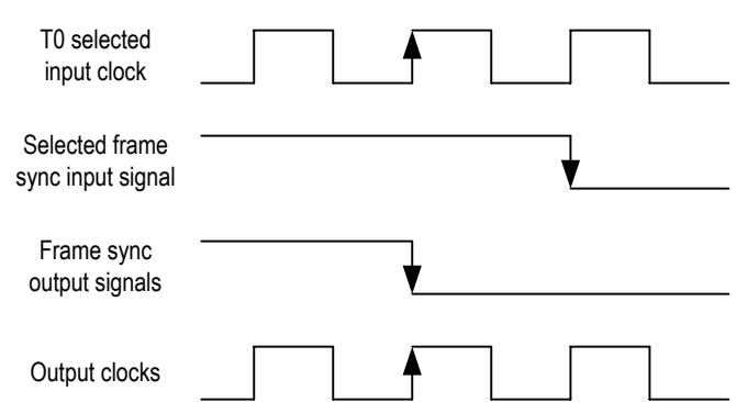
Figure 11. 1 UI Late Frame Sync Input Signal Timing
