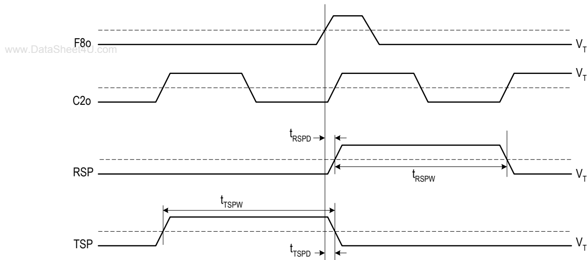
Figure - 13 Output Timing 2
