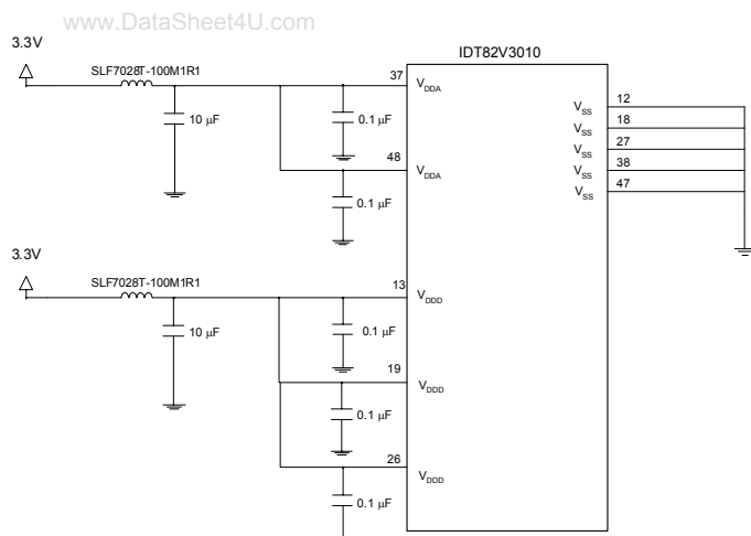
Figure - 10 IDT82V3010 Power Decoupling Scheme
