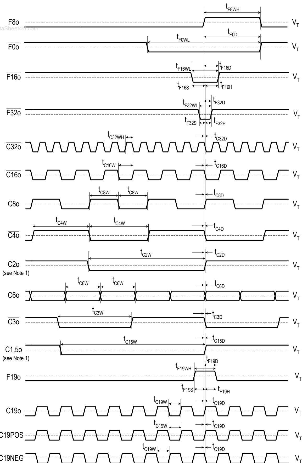
Figure - 13 Output Timing 1
