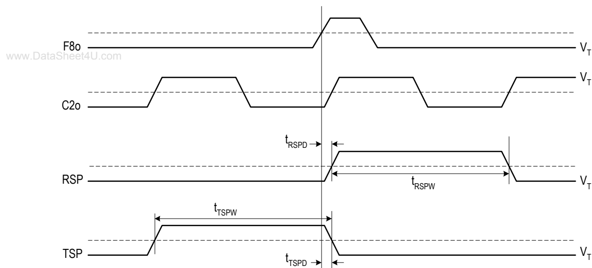
Figure - 14 Output Timing 2
