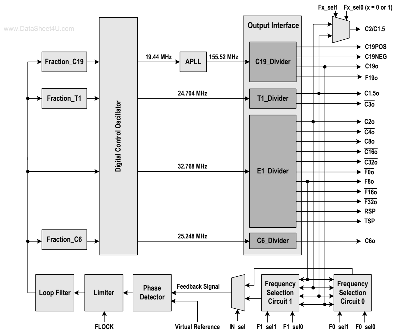
Figure - 7 DPLL Block Diagram
