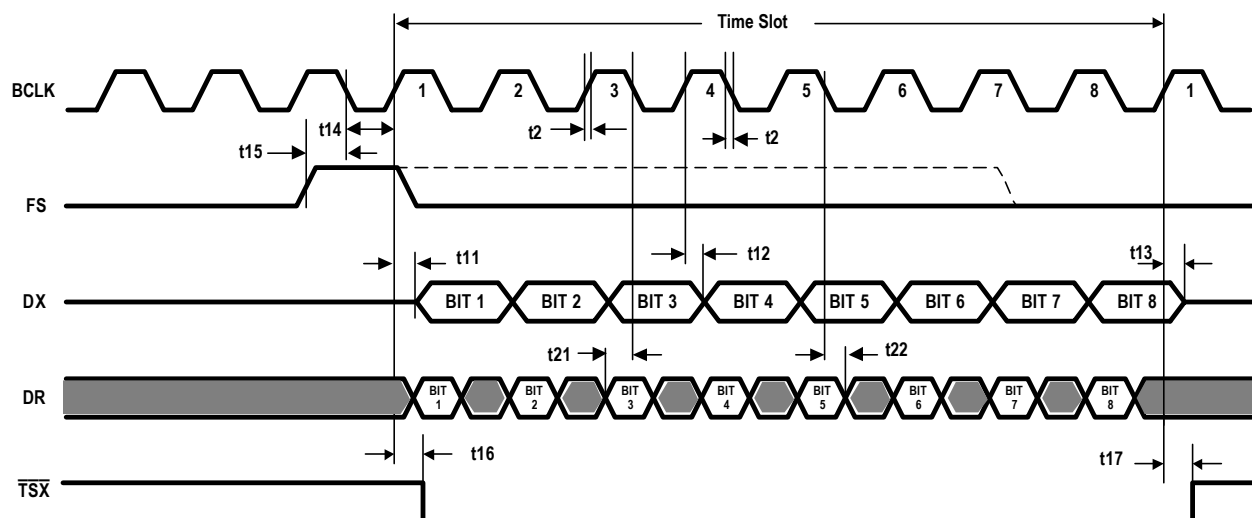
Figure 7. Transmit and Receive Timing in Delay Mode
