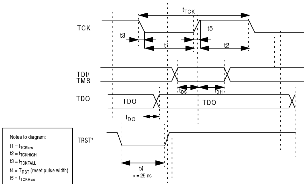
Figure 3 Standard JTAG Timing
