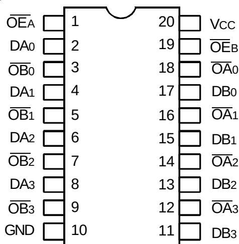
SOIC/ QSOP TOP VIEW
