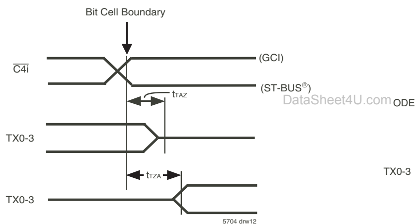
Figure 9. Serial Outputs and External Control
