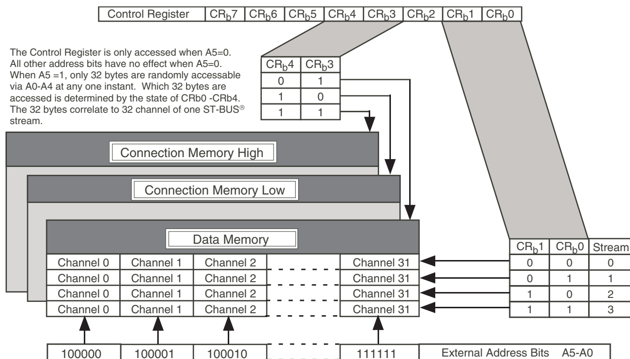
Figure 5. Addressing Internal Memories DataSheet4U.com
