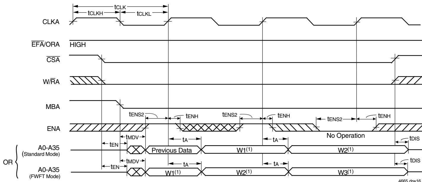
Figure 15. Port A Read Cycle Timing for FIFO02 (IDT Standard and FWFT Modes)
