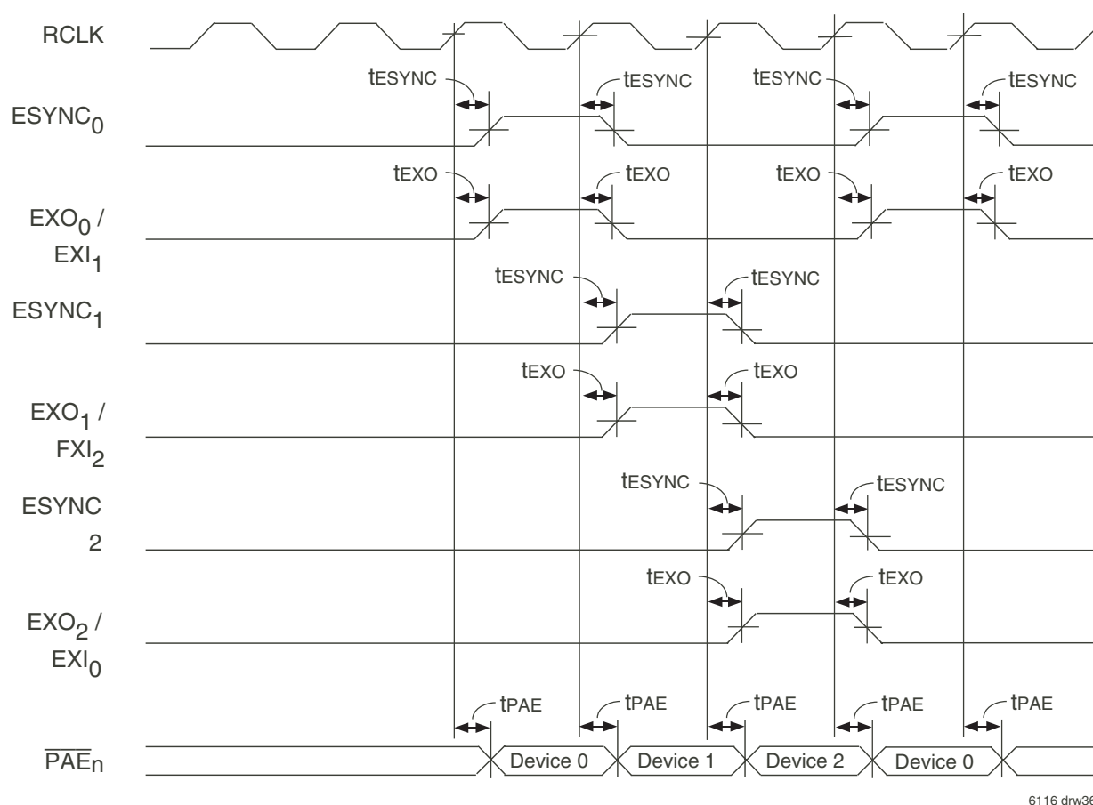
Figure 31. \overline{PAEn}/\overline{Pn} Bus - Polled Mode
