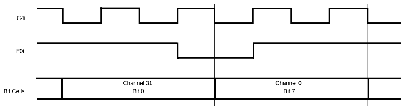
Figure 5. Frame Alignment
