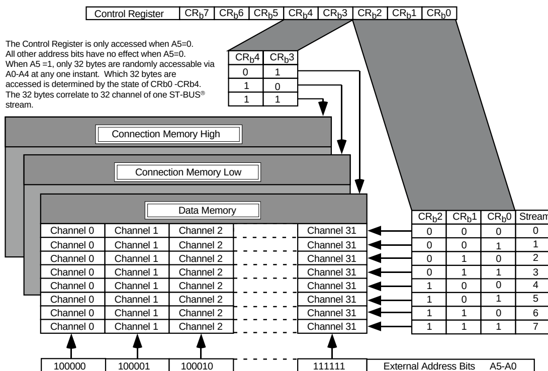
Figure 3. Address Mapping
