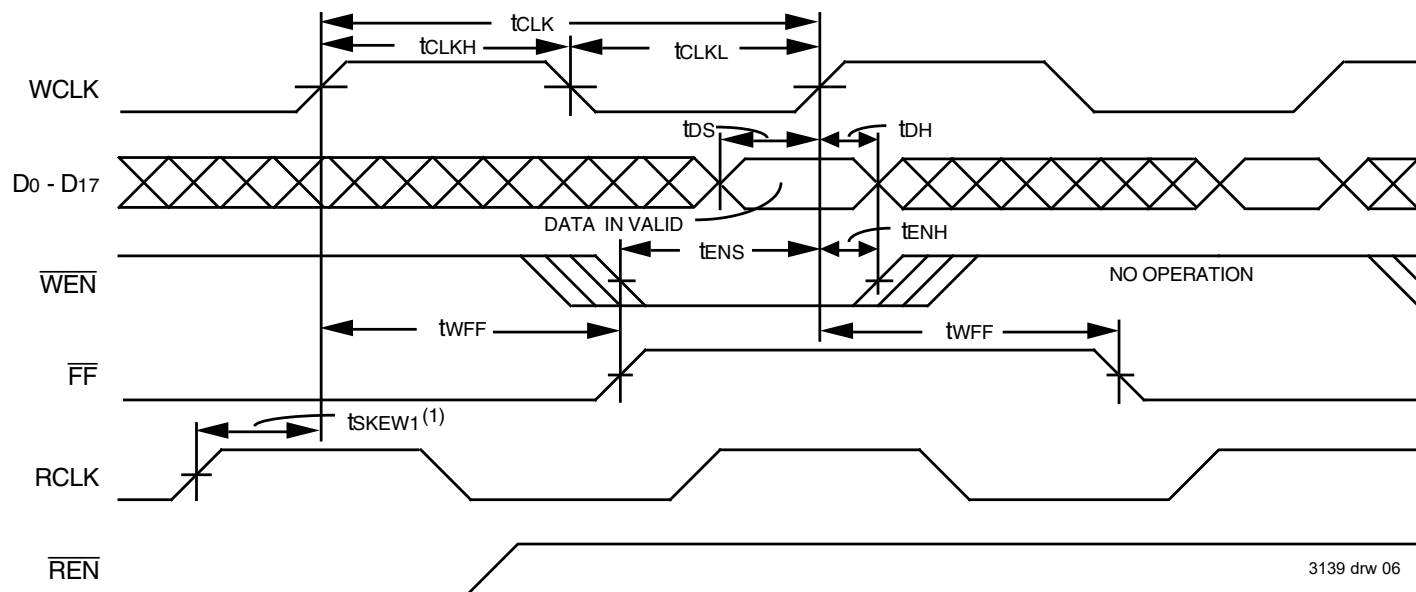
Figure 5. Reset Timing (2)
