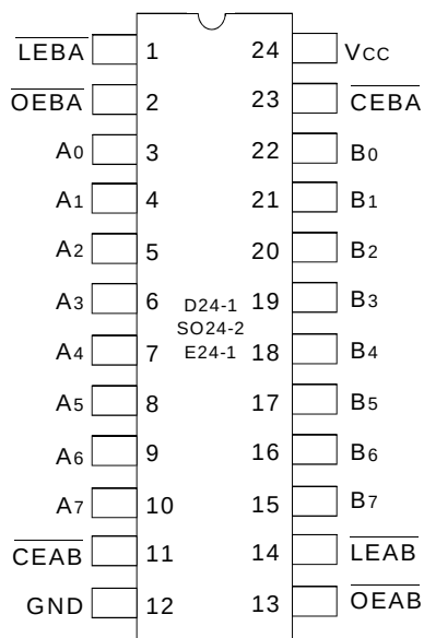
CERDIP/ SOIC/ CERPACK TOP VIEW
