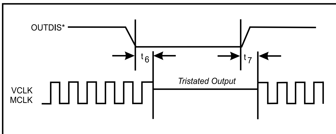
Tristated Timing
