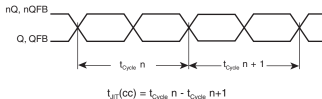
CYCLE-TO-CYCLE JITTER
