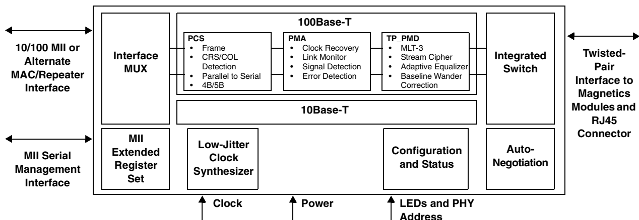
ICS1893CY-10 Block Diagram
