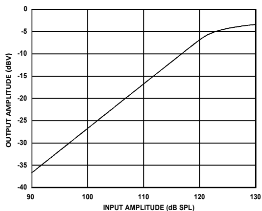
Figure 7. Linearity
