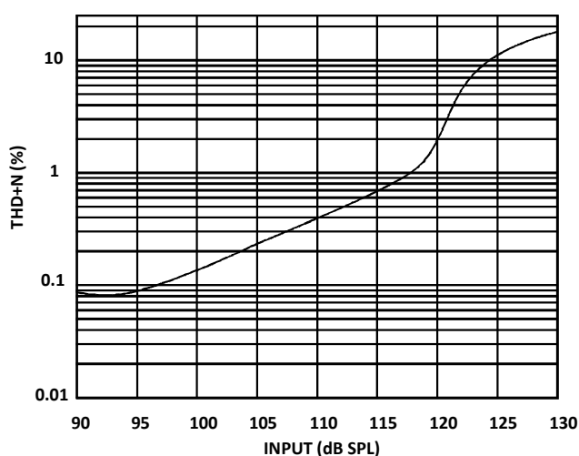
Figure 6. THD + N vs. Input Level
