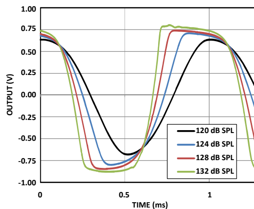
Figure 8 Clipping Characteristics
