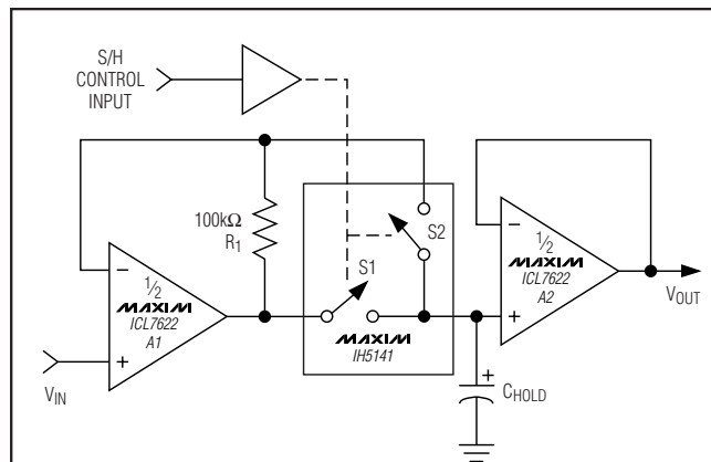
Figure 9. Low Droop Rate Sample and Hold—S2 improves accuracy and acquisition time by including the voltage drop across S1 inside the feedback loop of A1 during the hold phase. R1 closes the feedback loop of A1 during the hold phase. The droop rate is [I_{BIAS}(A2) + I_{LEAK}(S1) + I_{LEAK}(S2)]/C_{HOLD} .
