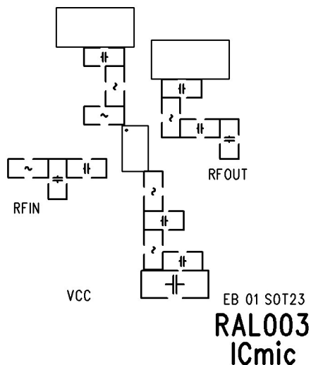
PCB SilkScreen
