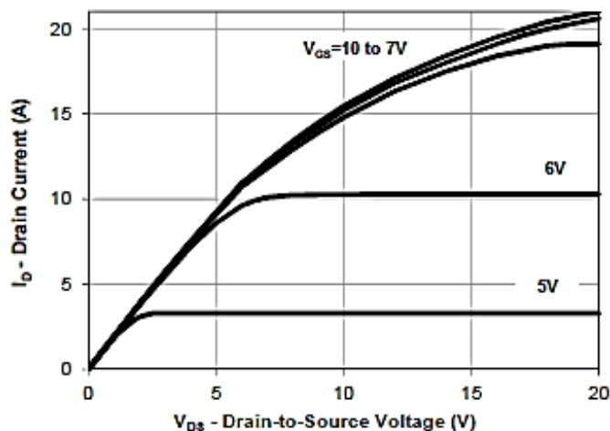
Output Characteristics
