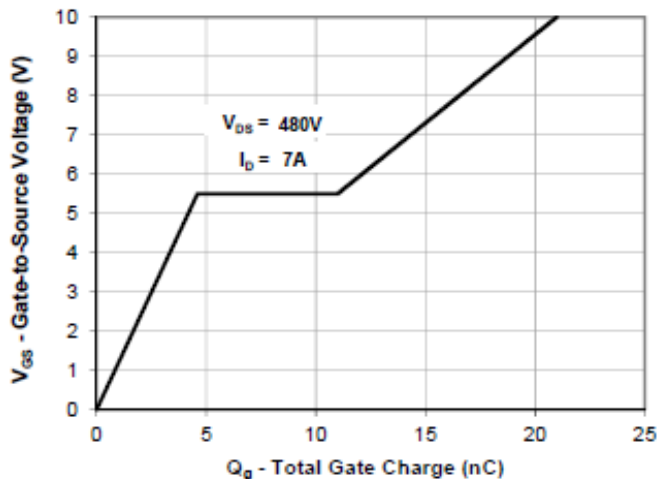
Gate Charge
