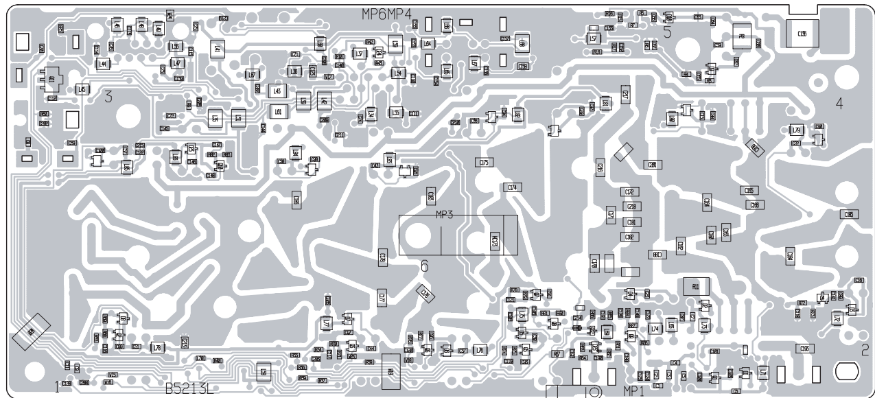
• HPF UNIT (BOTTOM VIEW)
