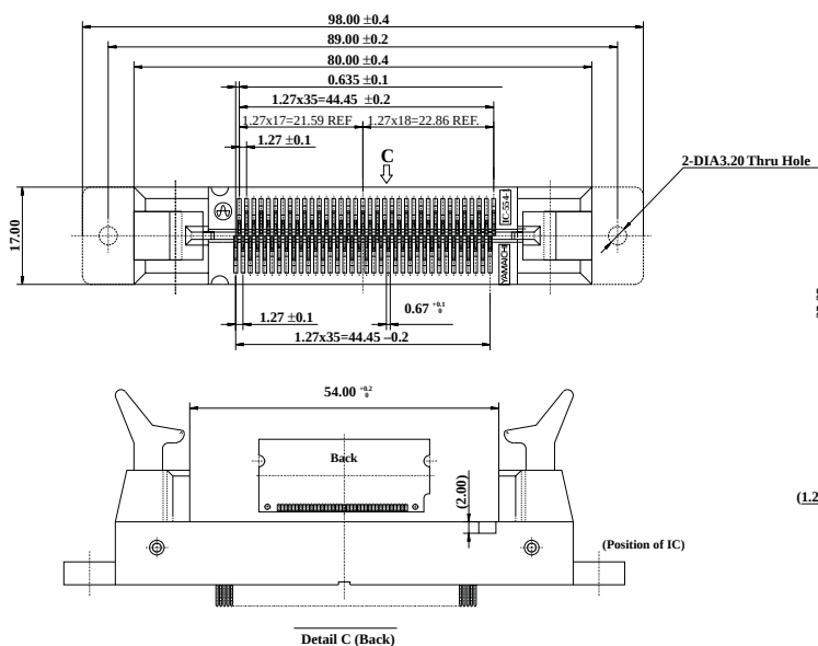
IC Device Dimensions (Reference Drawing)
