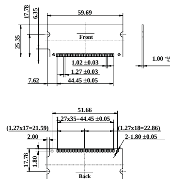
IC Device Dimensions (Reference Drawing)
