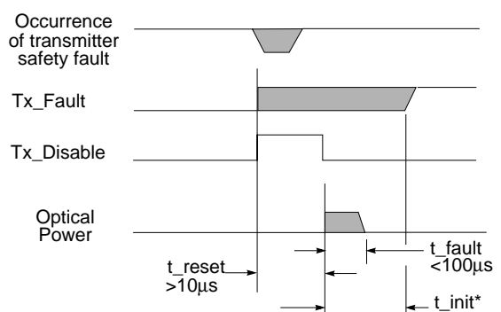
Unsuccessful Recovery from a Transmitter Safety Fault
