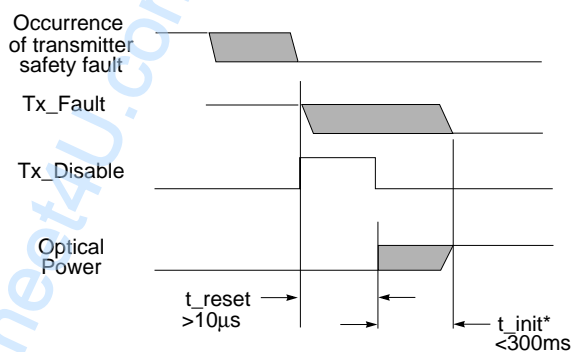
Successful Recovery from a Transmitter Safety Fault
