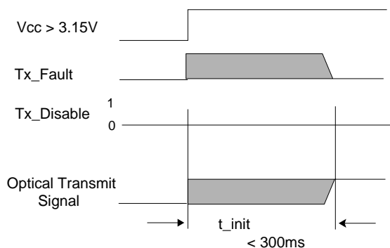
SFF-PGG-2125-SW/LW with Tx_Disable Deasserted
