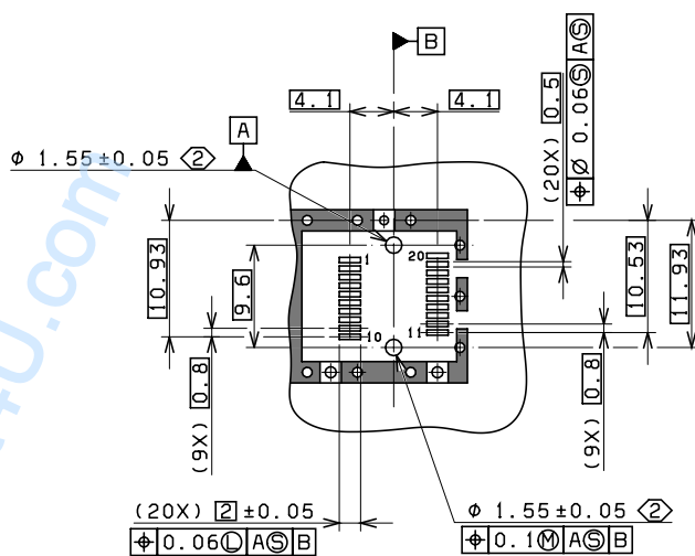
DETAIL X
