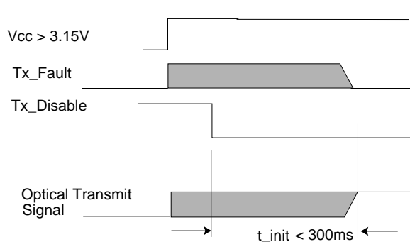
SFF-PGG-2125-SW/LW with Tx_Disable Asserted
